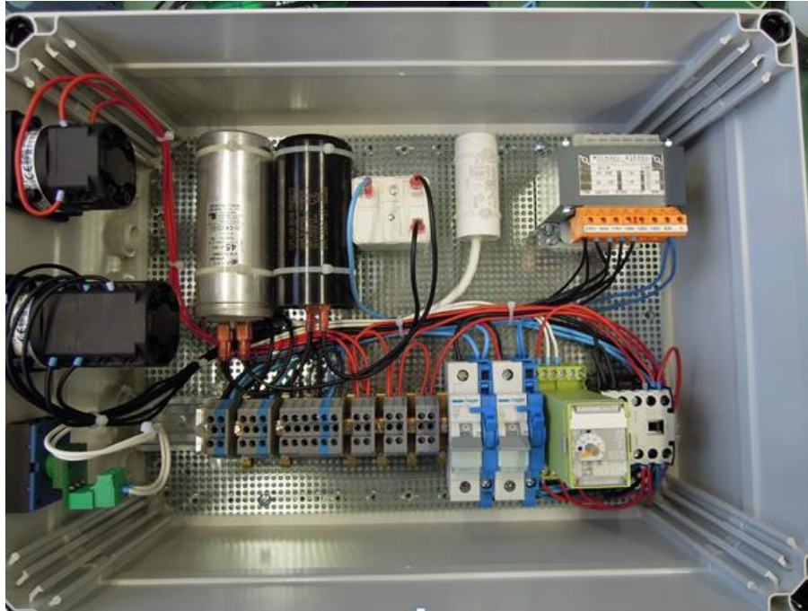
Completed circuit for a one-phase system
